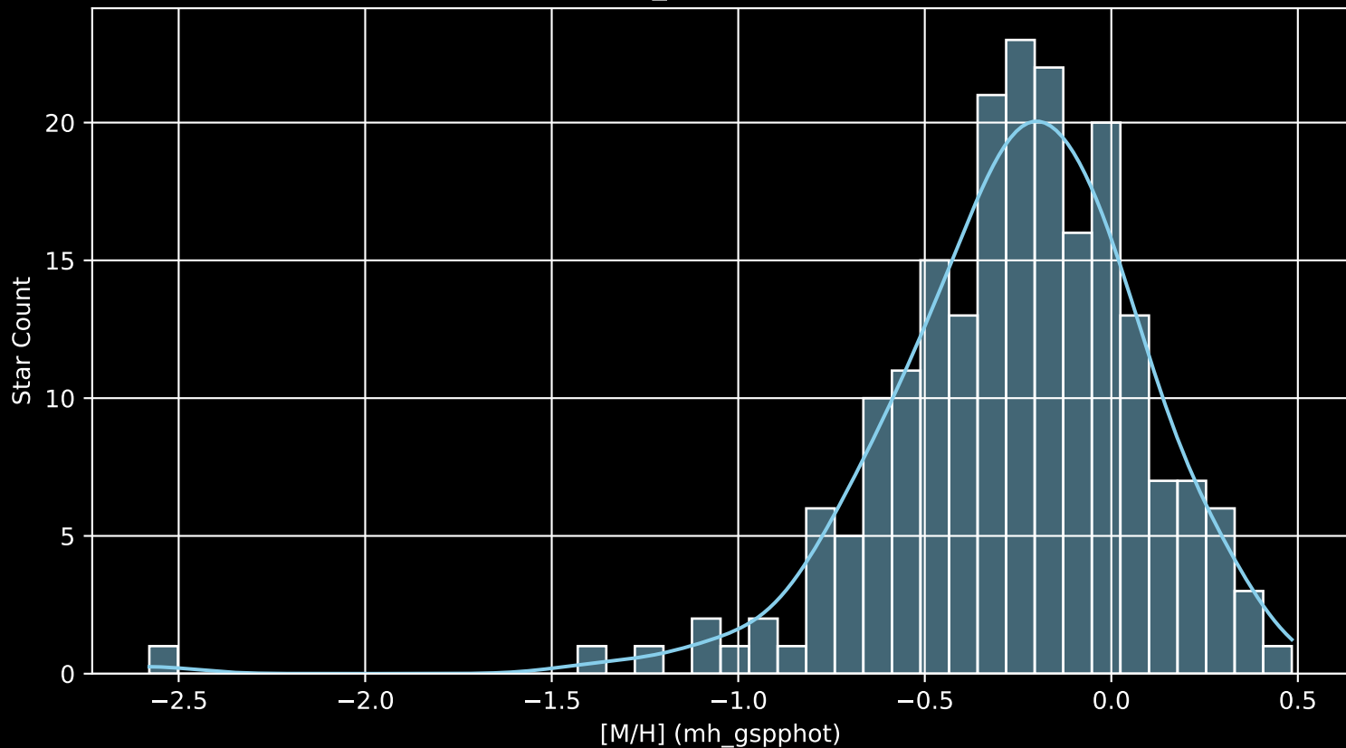
APOGEE DR17 Field: [K2_C12_070-63_btx [M/H] (mh_gspphot) (n= 208)
