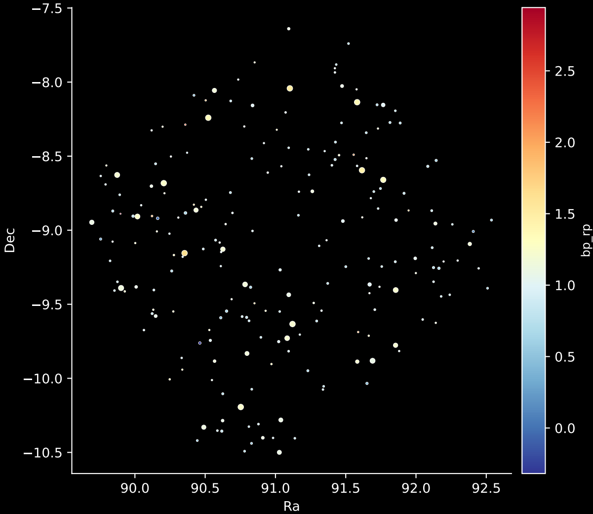
APOGEE DR17 Field: [K2_C12_070-63_btx] Stars: 209
