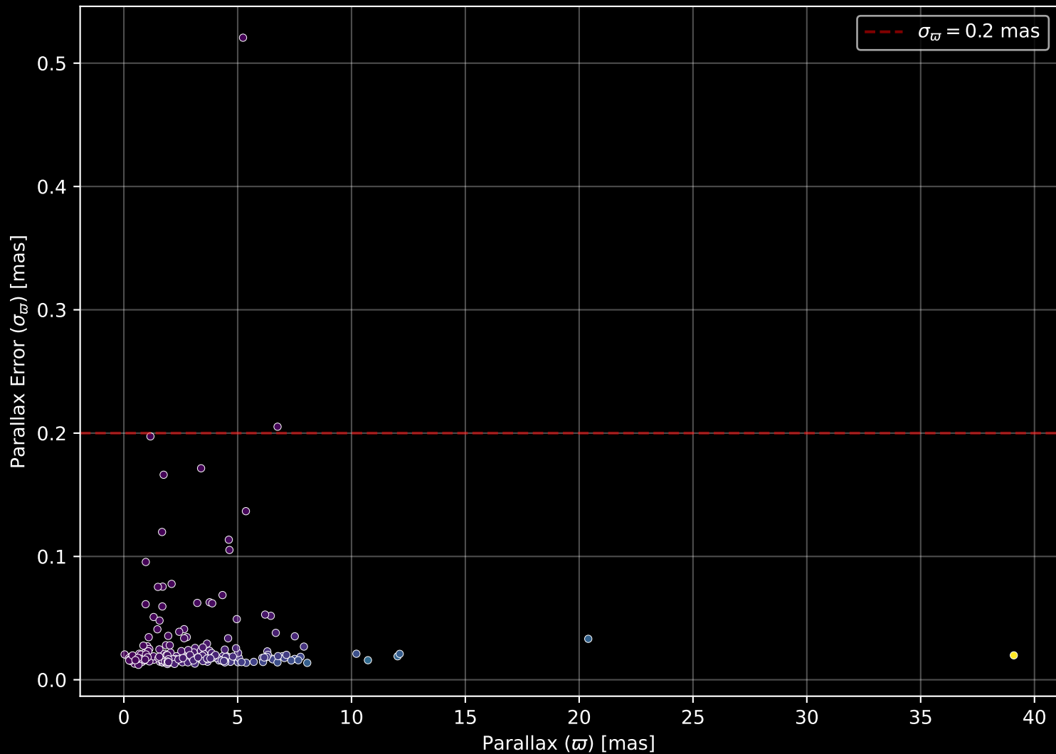
APOGEE DR17 Field: [K2_C12_070-63_btx] Parallax Quality (n= 209)
