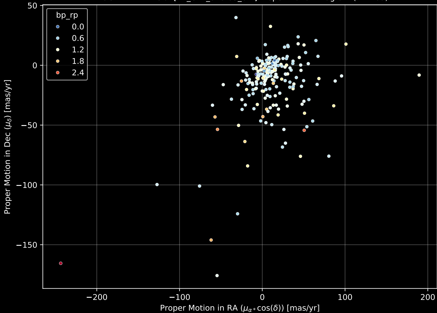
APOGEE DR17 Field: [K2_C12_070-63_btx] Proper Motion Diagram (n= 209)
