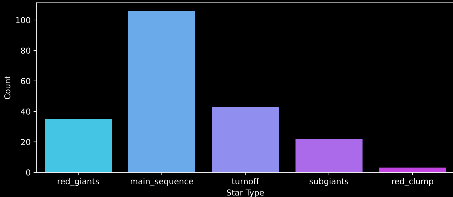
APOGEE DR17 Field: [K2_C12_070-63_btx] Count plot of Star Type
