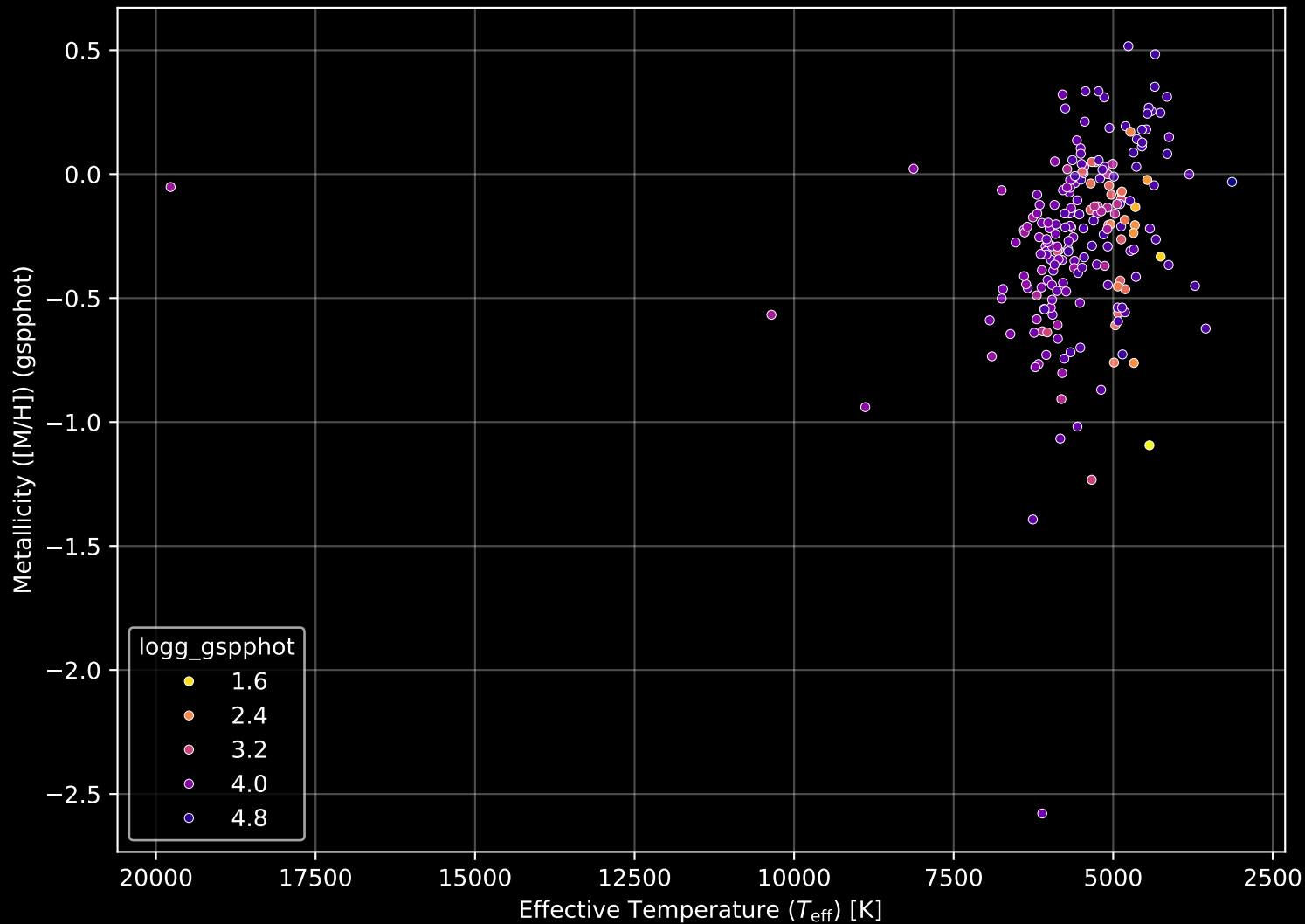
APOGEE DR17 Field: [K2_C12_070-63_btx] Stellar Population Parameters (n= 209)
