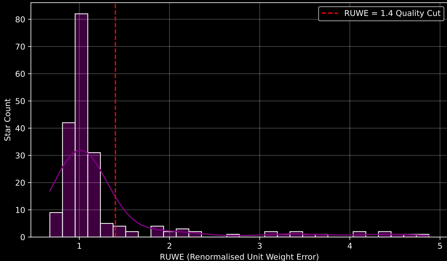
GAPOGEE DR17 Field [K2_C12_070-63_btx] RUWE Distribution (n= 201)
